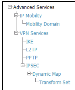
Figure 6 Device Setup > Alcatel-Lucent Configuration > Advanced Services Navigation
