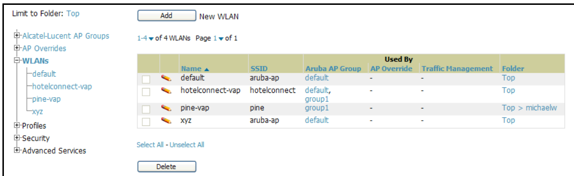
Figure 19 Device Setup > Alcatel-Lucent Configuration > WLANs Page Illustration
