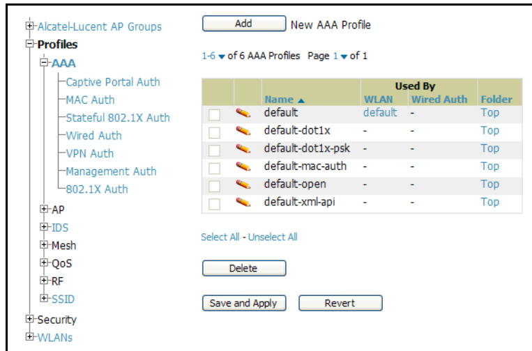
Figure 36 AAA Profiles Page of Alcatel-Lucent Configuration
