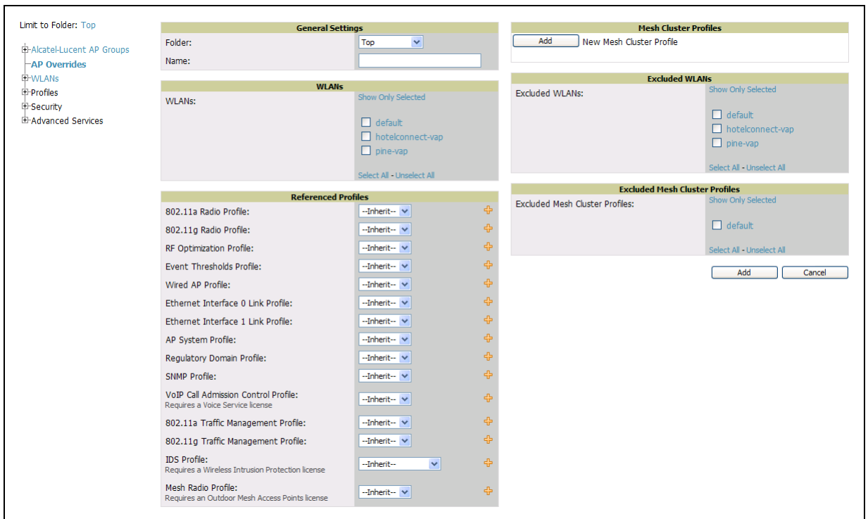
Figure 24 AP Overrides Add or Edit Page Illustration (Non-scrolling View)
