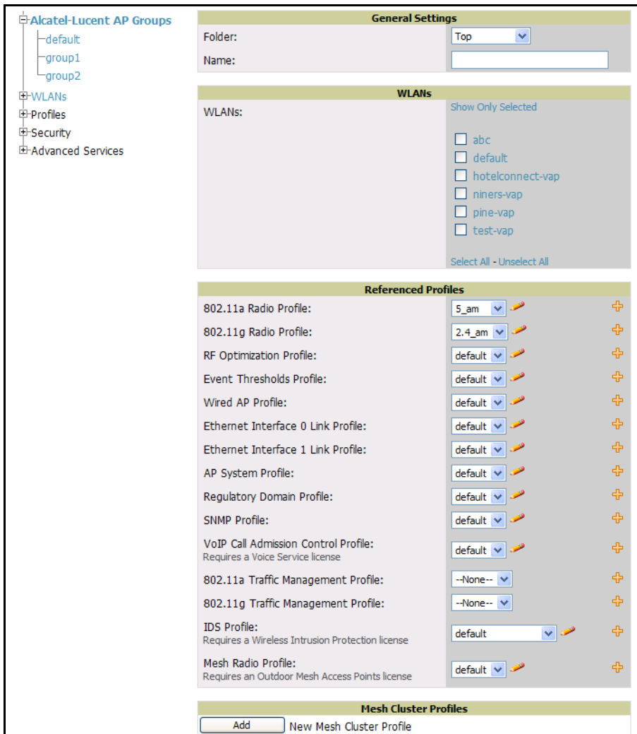
Figure 18 Device Setup > Alcatel-Lucent Configuration, Group Details Page Illustration
