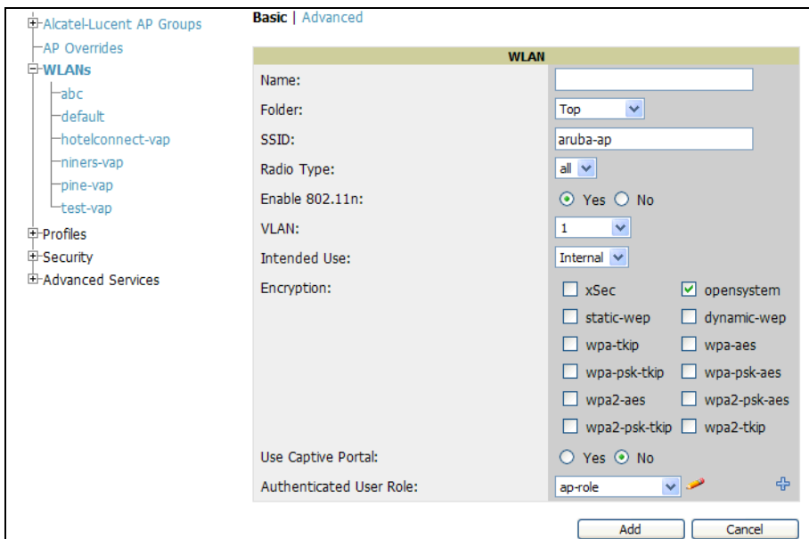
Figure 20 WLANs > Basic Page Illustration
