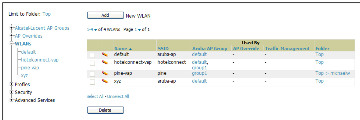
Figure 31 WLANs Navigation and Page
