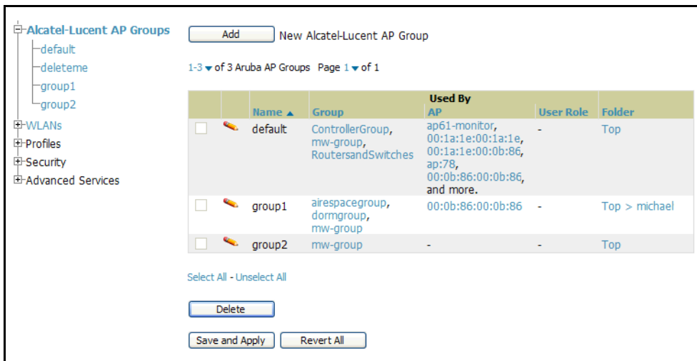
Figure 17 Device Setup > Alcatel-Lucent Configuration > AP Groups Page Illustration
