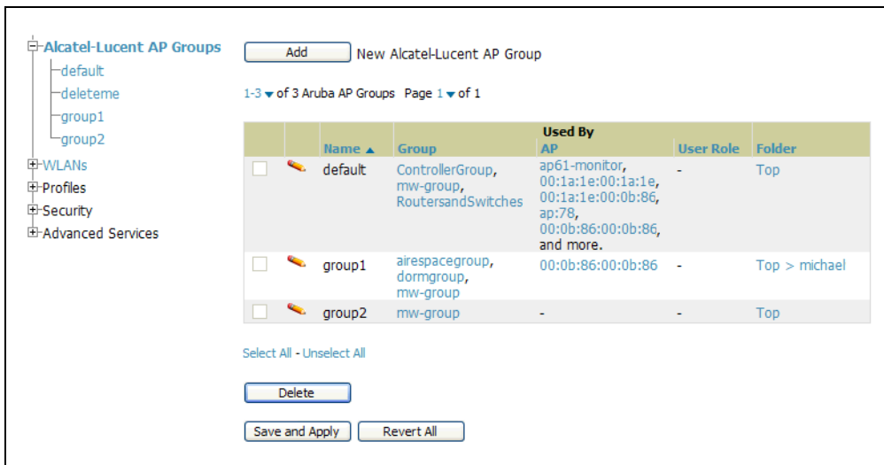
Figure 12 Device Setup > Alcatel-Lucent Configuration > Alcatel-Lucent AP Groups Page
