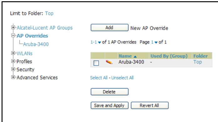
Figure 32 AP Overrides Page
